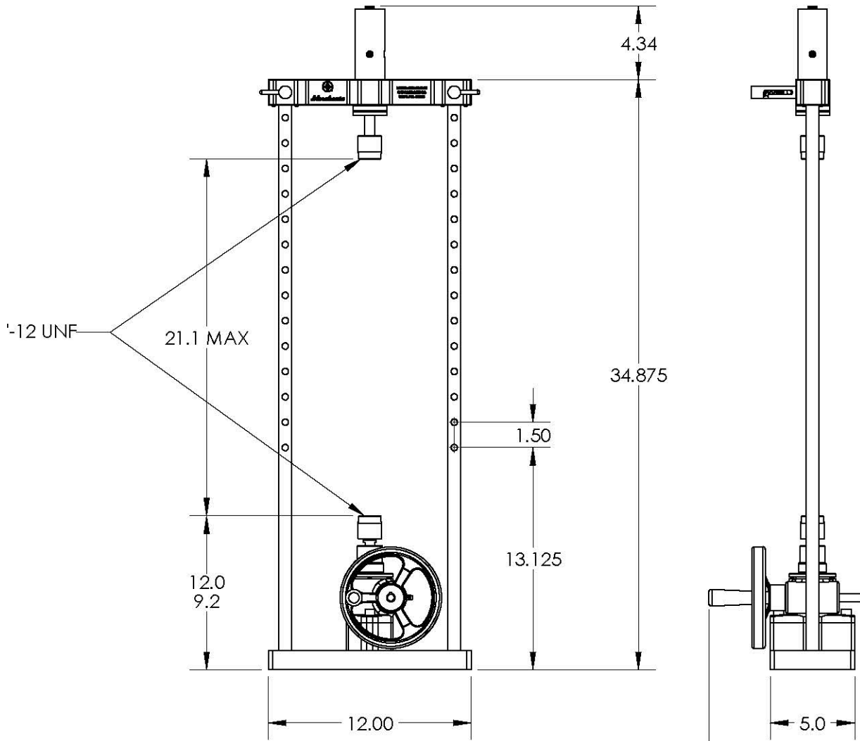
Figure 5: Dimension Guide for PCM2K-2 Machine Model
