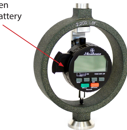
Figure 4: Battery Compartment in Morehouse Digital Force Gauges
