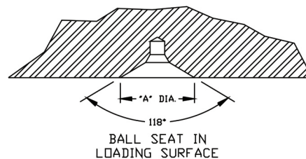
Figure 2: Ball Seat Dimensions
