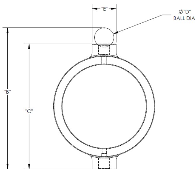
Figure 2: Ball Seat Dimensions
