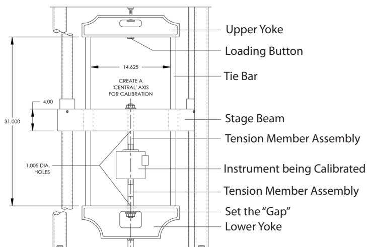
Figure 5: Tension Calibration
