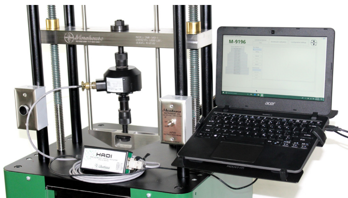
Figure 8: Control and Automate with the Deadweight Calibration System (DCS)
