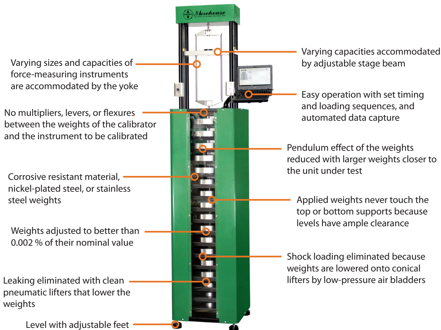
Figure 1: Deadweight Calibrating Machine
