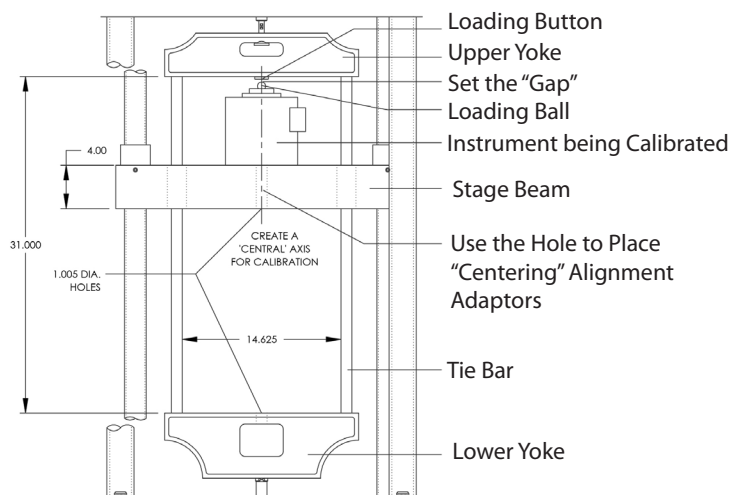
Figure 4: Compression Calibration
